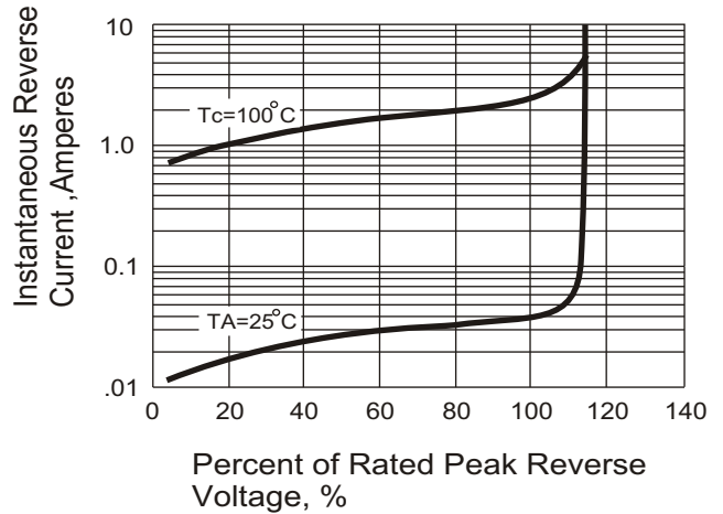
Fig. 4 Typical Revers Characteristics
